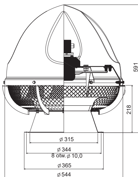
Wentylator dachowy SMART-EC-4000
