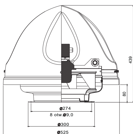
Wentylator dachowy SMART-EC-1300
