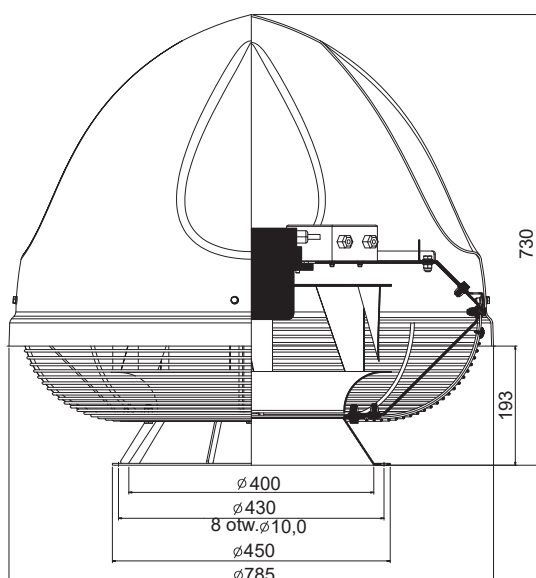
Wentylatory dachowe SMART-EC-6200
