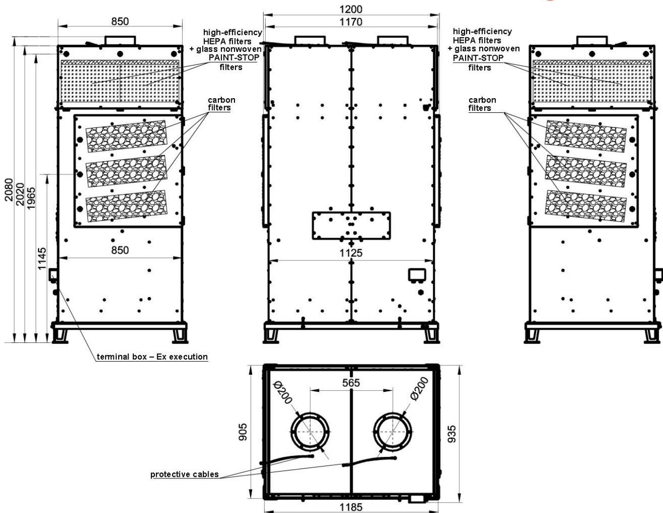
Fig. No.2 – SMOG Filter-2400/Ex – Structure and dimensions
