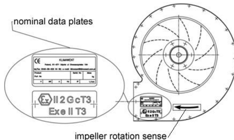
Fig. No. 4 – Placement of the nominal data plates and the arrow of the correct impeller rotation sense
