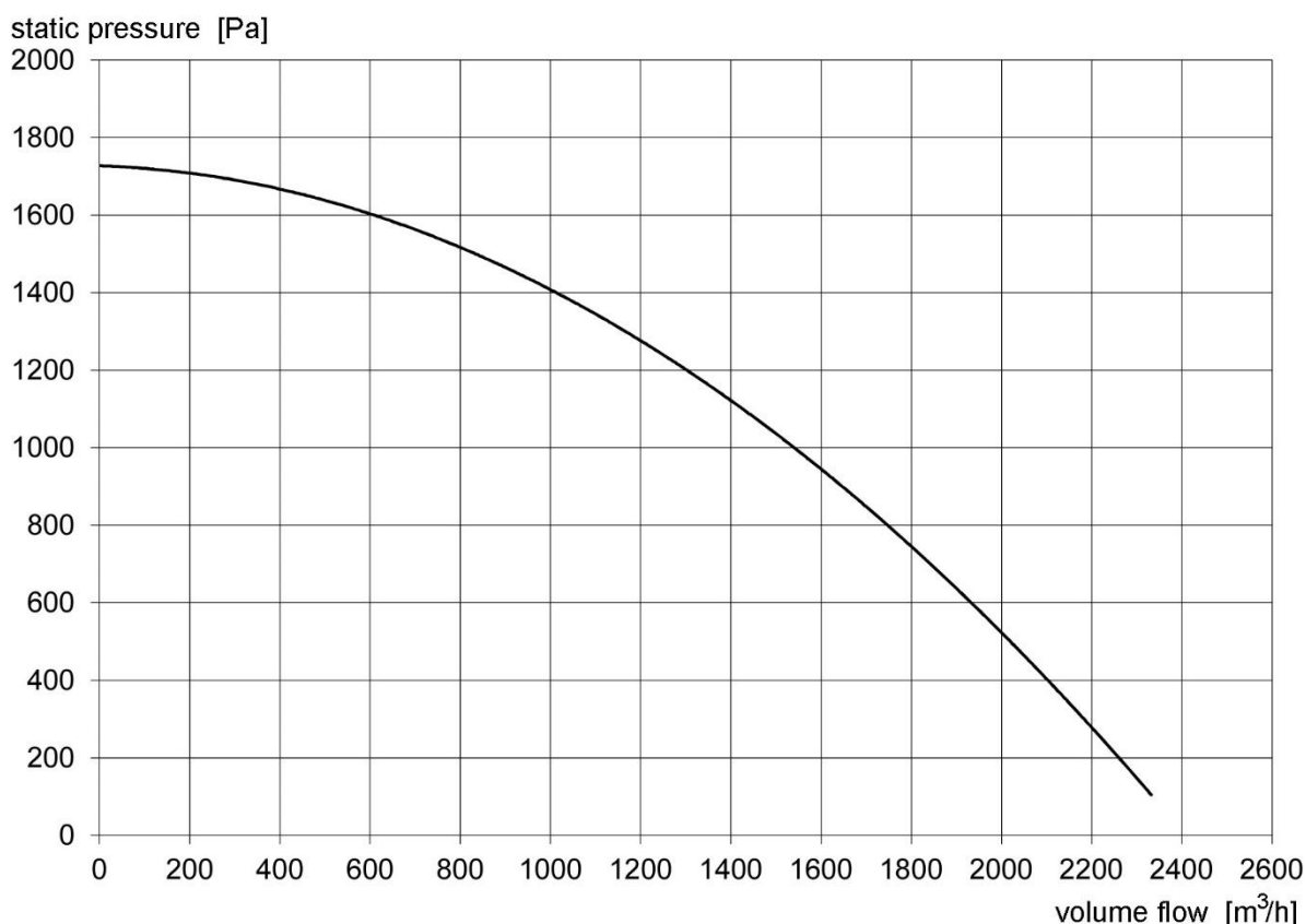
Fig. No. 1 – SMOG Filter-2400/Ex – Flow chart
