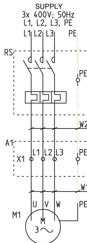
Fig. No.3 – SMOG Filter-2400/Ex Connection Diagram
