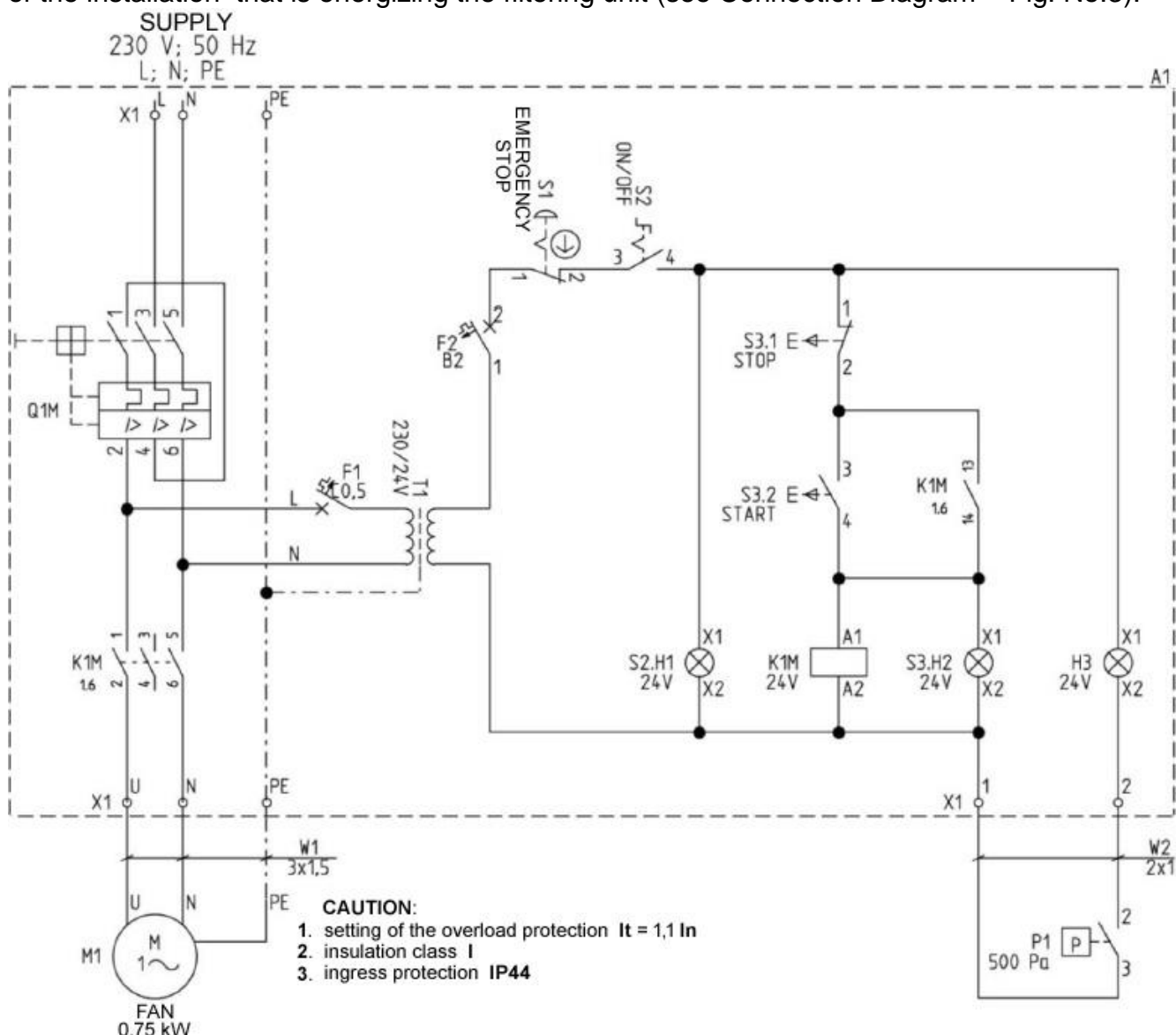
Fig. No.3 – MISTOL DUST-1000 – Connection Diagram
