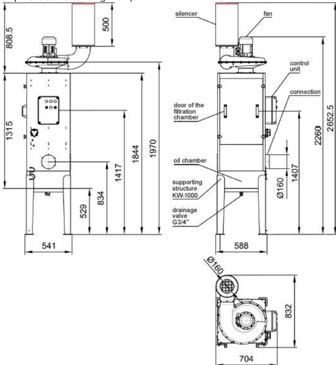
Fig. No.2 – MISTOL DUST-1000 – Structure and dimensions
