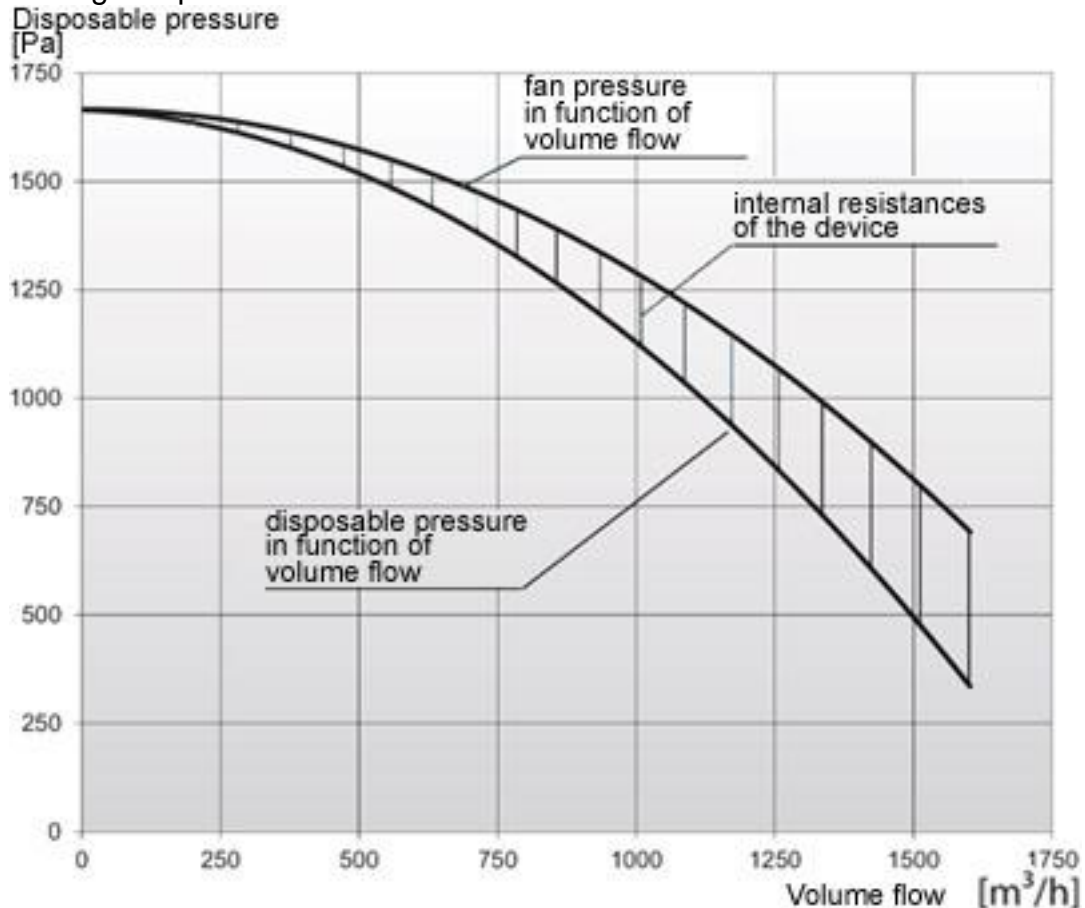
Fig. No.1 – MISTOL DUST-1000 – Flow chart
