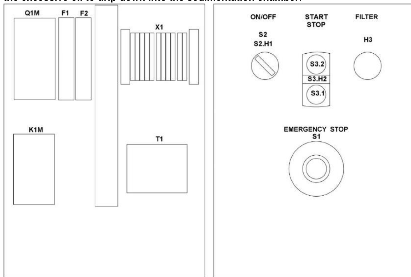
Fig. No.4 – MISTOL DUST-1000 – control unit
