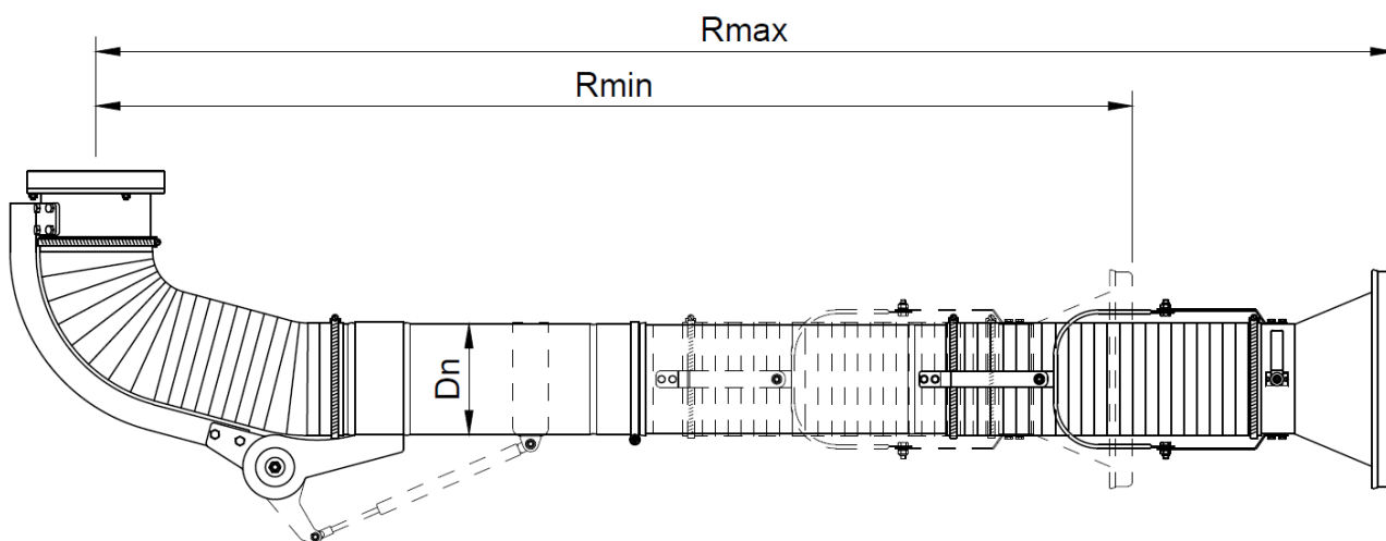
Rys. 2 TELERGO-L-2-2000; 2400
