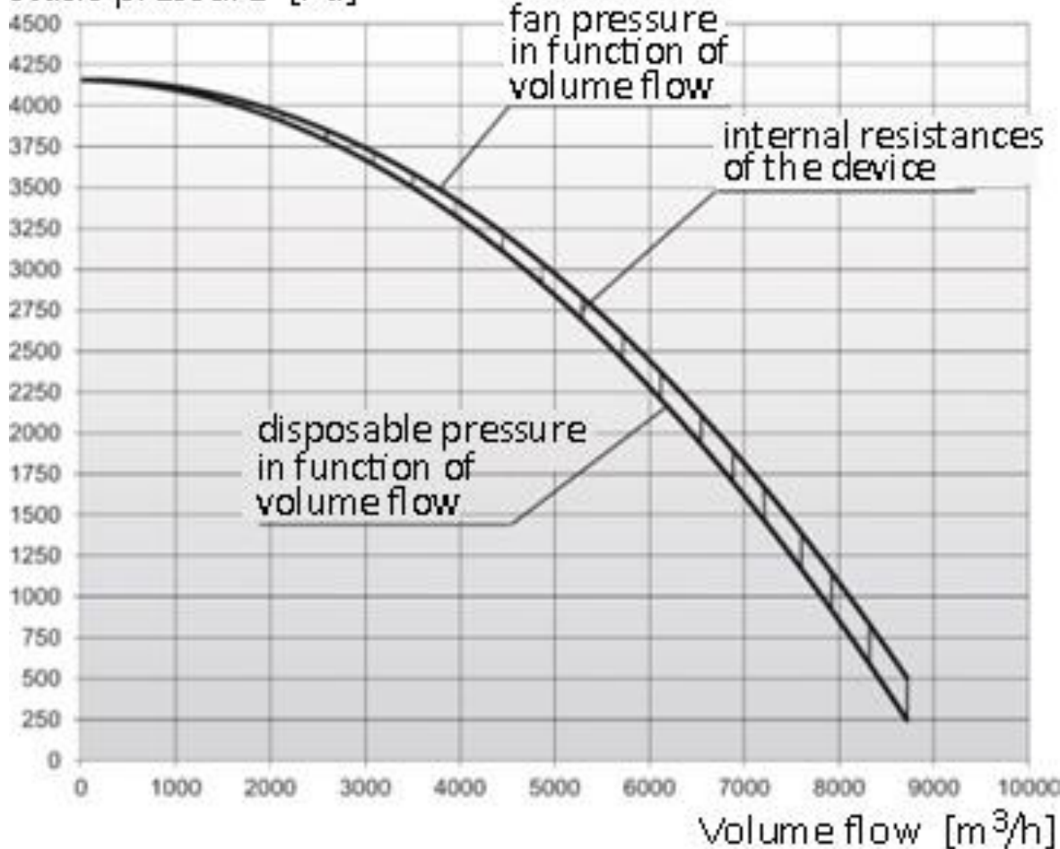
Fig. No.1 – Flow chart of the Oil Mist Separator MISTOL MIX-5000
