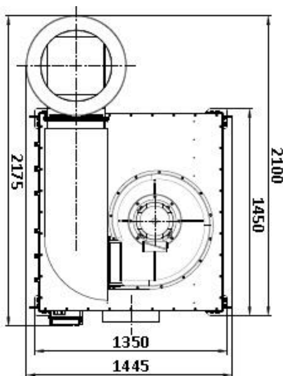
Fig. No.2a – Structure and dimensions of the Oil Mist Separator MISTOL MIX-5000
