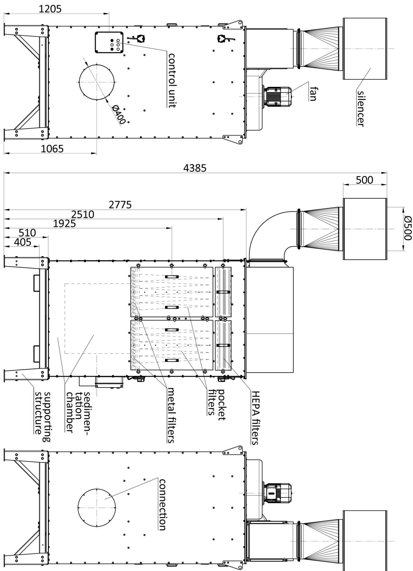
Fig. No.2b – Structure and dimensions of the Oil Mist Separator MISTOL MIX-5000
