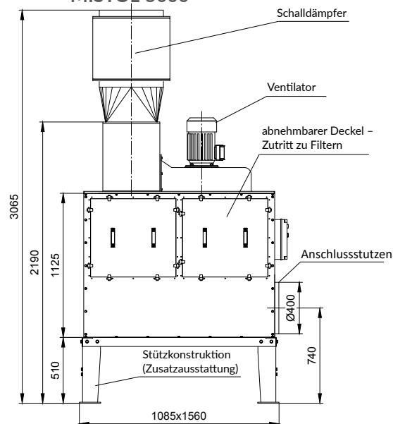
MISTOL-5000
