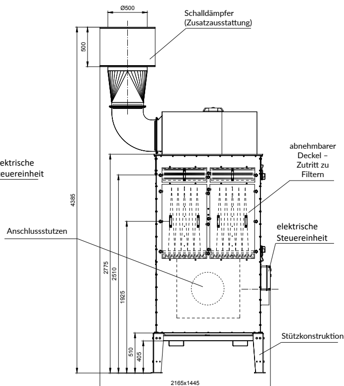
MISTOL MIX-5000
