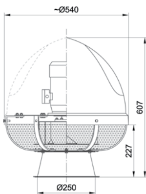
Dachventilator SMART-250/3000-SN
