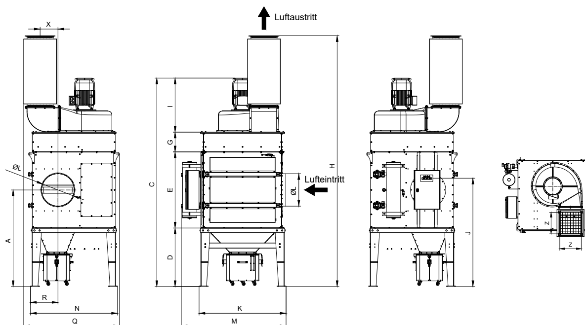
UFO-A-10000-N
