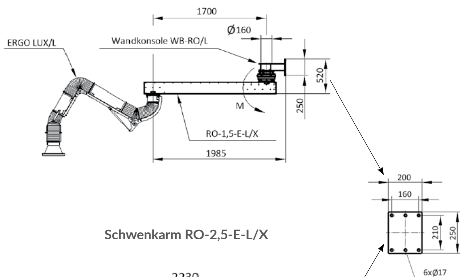
Schwenkarm RO-1,5-E-L/X
