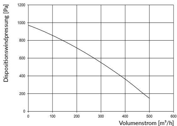
SMOG Filter-1200
