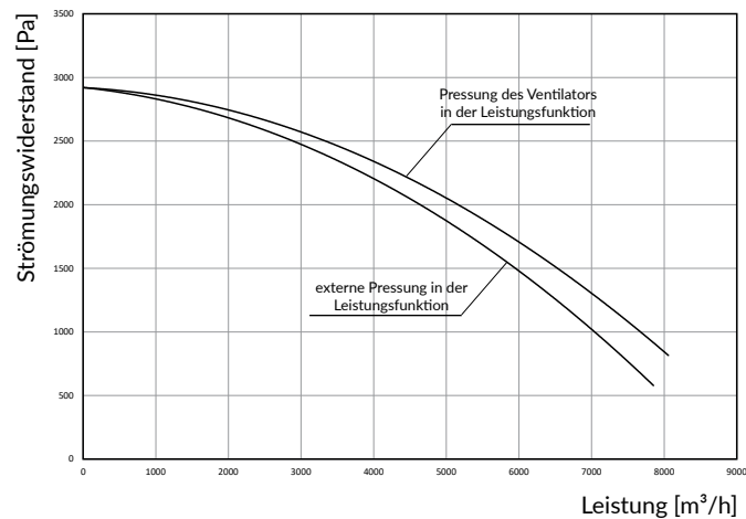
PROTON-8000
