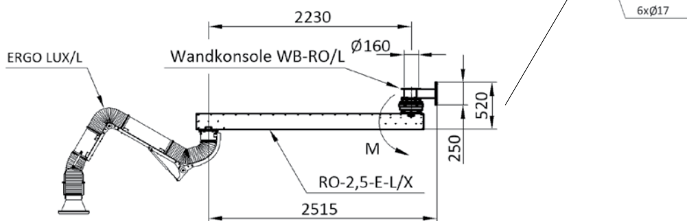
Schwenkarm RO-2,5-E-L/X
