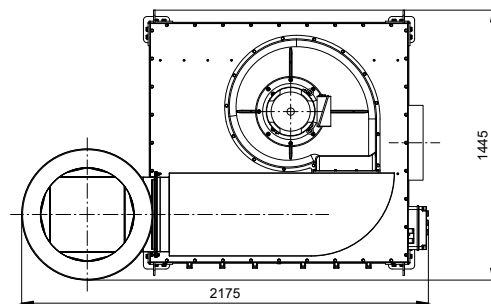
MISTOL MIX-5000
