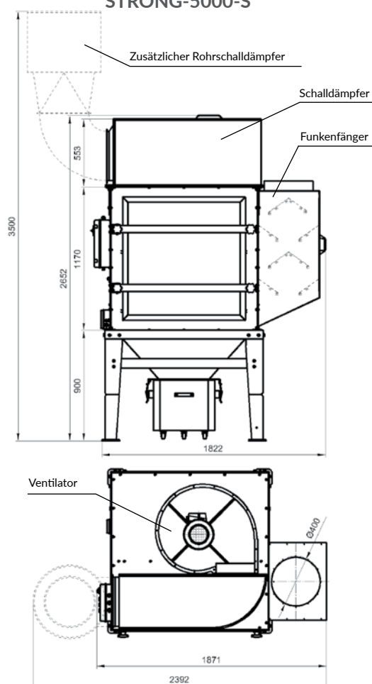
STRONG-5000-S
