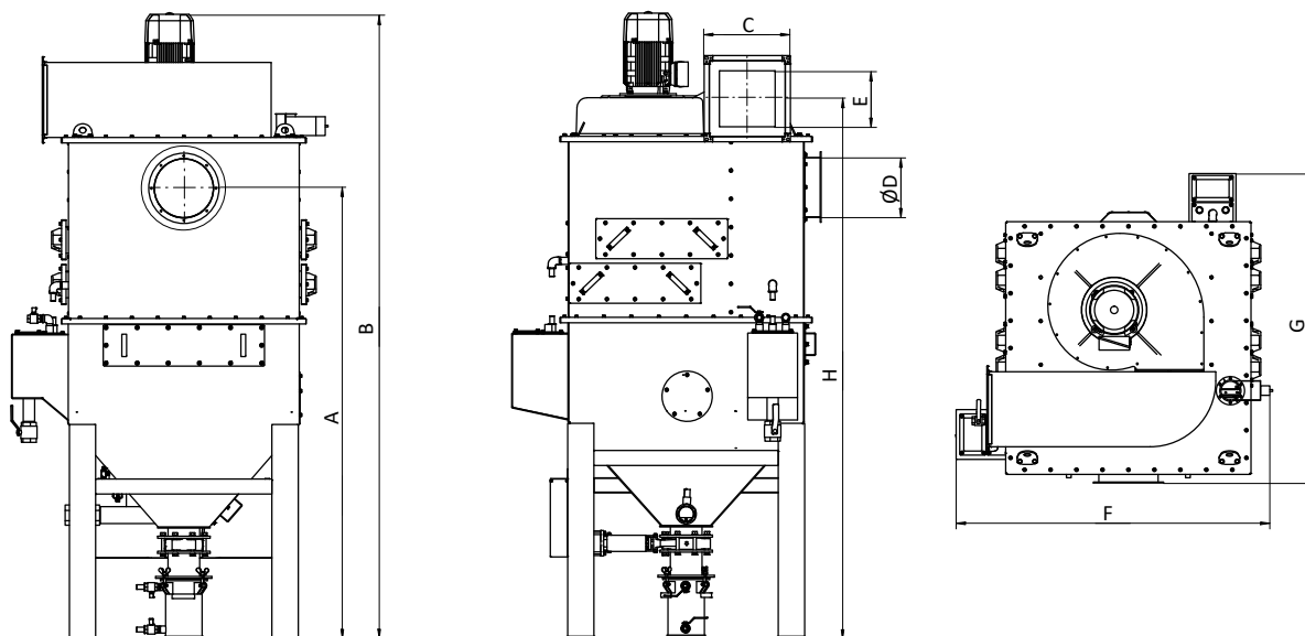
WET-ALU-4000/Ex
